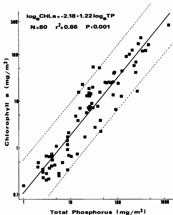
Fig. 2. Relation between mid-summer chlorophyll-a and total phosphorus concentration for 80 Argentinian lakes and reservoirs with \text{TN} : \text{TP} > 22 (molar basis). Broken line is the 95 % predictive confidence interval.
