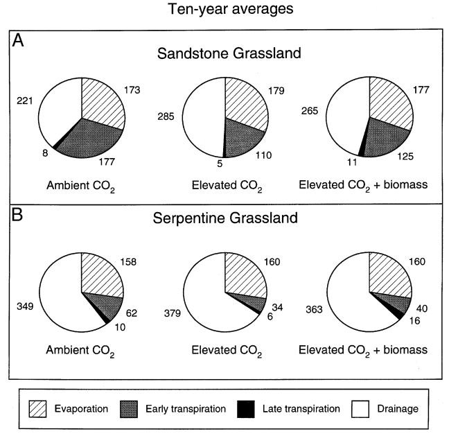
Fig. 3 Ten-year averages of simulated water fluxes (mm H 2 O yr -1 ) for the A sandstone and B serpentine grasslands. The three treatments are ambient CO 2 ( A ), elevated CO 2 ( E ) as simulated by reduced transpiration, and elevated CO 2 + biomass (20% more early-season annuals and a 3-fold increase in late-season annuals)
