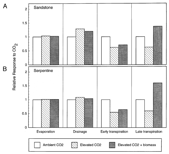
Fig. 4 Relative changes from ambient CO 2 in soil evaporation, soil drainage, early-season transpiration, and late-season transpiration in elevated CO 2 ( E ) and elevated CO 2 + biomass ( E+B ) for the A sandstone and B serpentine grasslands. Values are based on the 10-year averages from Fig. 3; the eight ambient CO 2 bars all equal one
