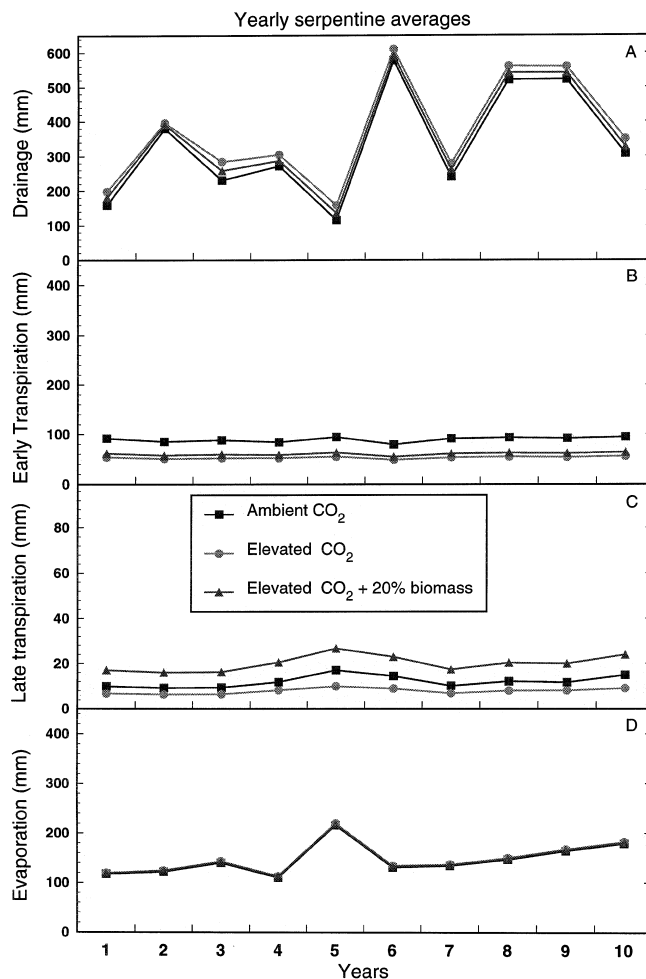
Fig. 6 Yearly values (mm H 2 O) for A soil drainage, B early-season transpiration, C late-season transpiration, and D soil evaporation in the serpentine grassland at ambient CO 2 , elevated CO 2 (E) and elevated CO 2 + biomass (E+B)
