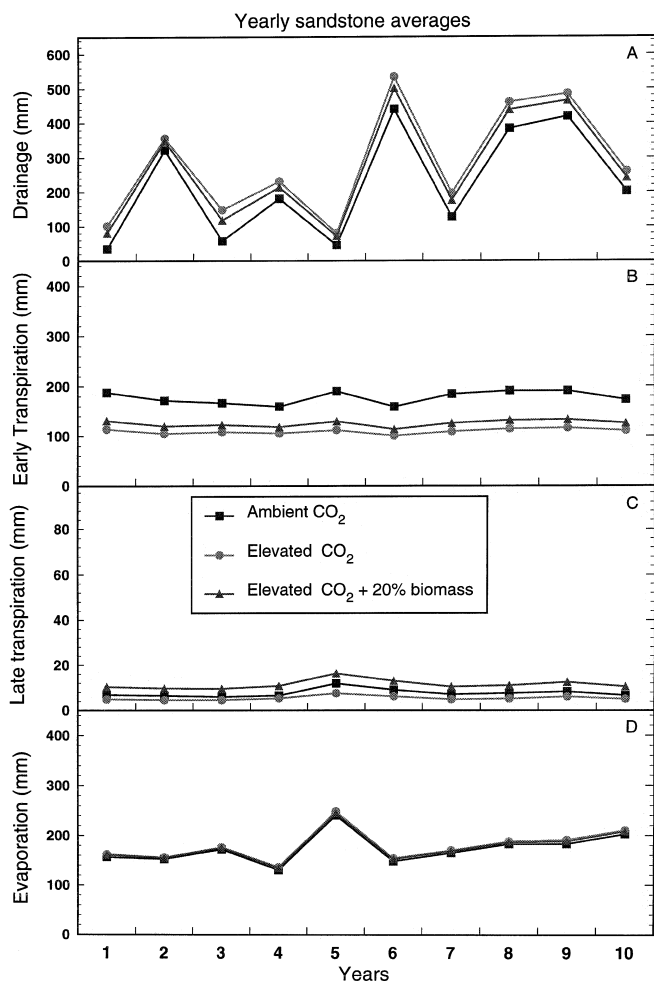
Fig. 5 Yearly values (mm H 2 O) for A soil drainage, B early-season transpiration, C late-season transpiration, and soil evaporation in the sandstone grassland at ambient CO 2 , elevated CO 2 (E) and elevated CO 2 + biomass (E+B)
