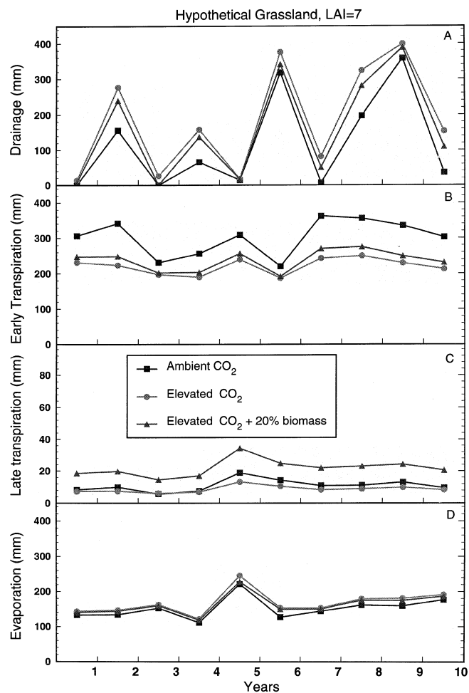
Fig. 7 Yearly values (mm H 2 O) for A soil drainage, B early-season transpiration, C late-season transpiration and D soil evaporation in a hypothetical grassland with LAI = 7 at ambient CO 2 , elevated CO 2 (E) and elevated CO 2 + biomass (E+B)
