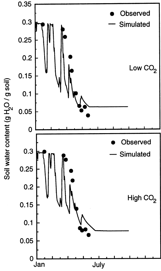
Fig. 2 Simulated and observed soil moisture in 1993 for the sandstone grassland in ambient and elevated CO 2 . Observed moisture values are for the upper 15 cm of soil taken with a time-domain reflectometry system
